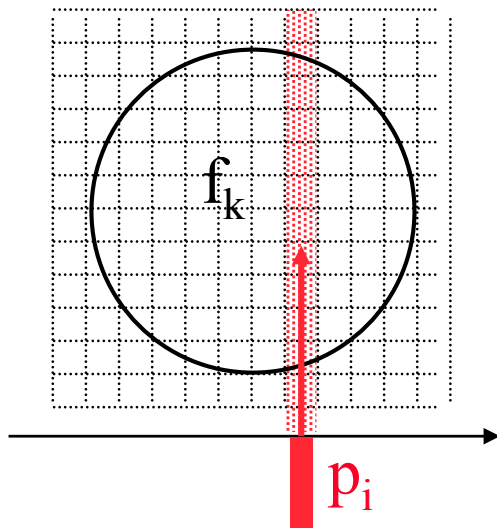
Backprojection without prior
